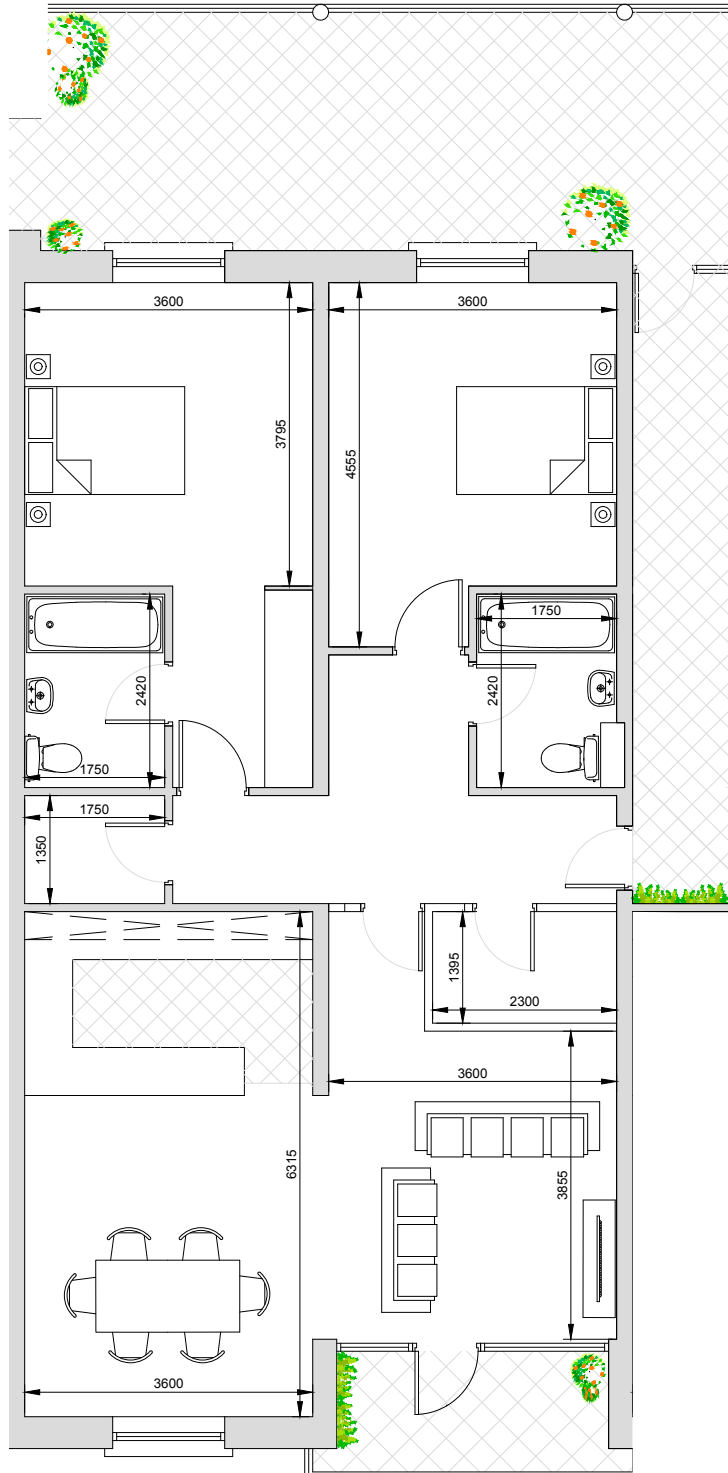
APARTMENT 8 - 1st Floor, 2 Bed, 101.2m 2
