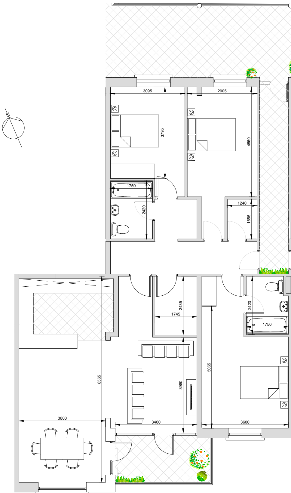
APARTMENT 10 - 1st Floor, 3 Bed, 126.9m 2
