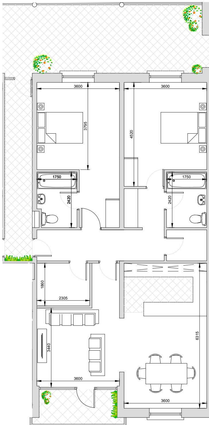
APARTMENT 11 - 1st Floor, 2 Bed, 101.2m 2
